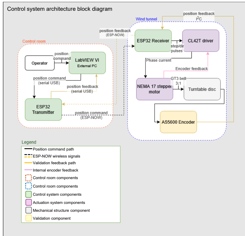
Figure 6.1: Turntable control system architecture block diagram
