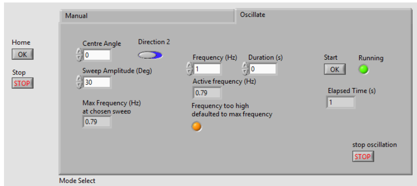
Figure D. 5: Oscillation control max frequency control
